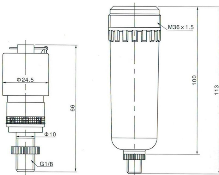
Dimensional drawing of water cup conneting part
