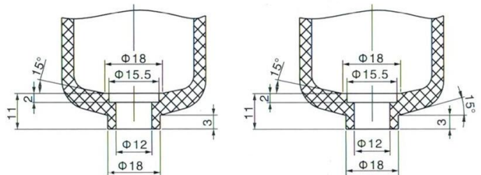
Dimensional drawing of water cup connecting part
